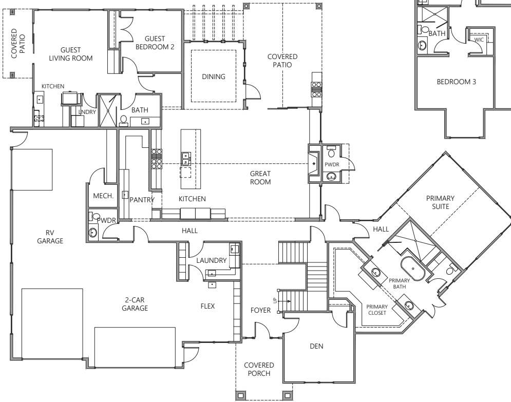
MAIN LEVEL
